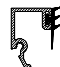
WQ55 28mm BEAD FLUSH SASH
