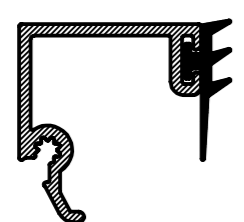
WQ50 28mm BEAD
