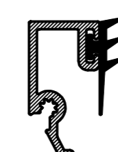
WQ56 32mm BEAD FLUSH SASH
