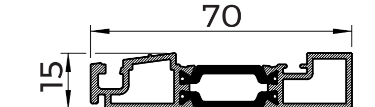
WT02 OPEN OUT LOW THRESHOLD
