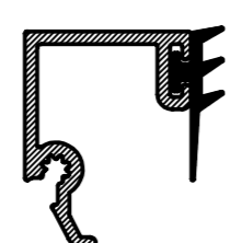
WQ51 32mm BEAD
